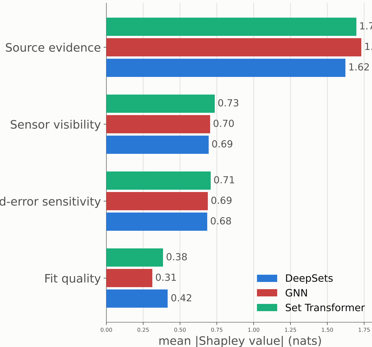
A. Mean absolute contribution
